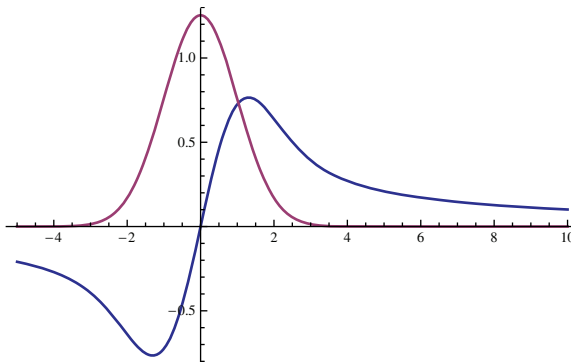
FIGURE 1.1. The imaginary part and the real part of \Psi^{\text{Catalan}}(x, 1) . For x \gg 0 , the imaginary part dies down, and only the real part has a non-trivial asymptotic expansion. Thus \text{protect}(1.27) is a series with real coefficients.
