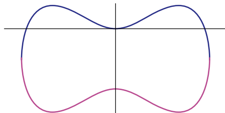
FIGURE 1.3. The spectral curve of the fifth example, which is non-singular. The corresponding quantum curve has two regular singular points at x = \pm 1 , and a class 1 irregular singular point at x = \infty .
