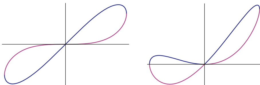
FIGURE 1.2. The spectral curves of the second and the fourth examples. The horizontal line is the divisor C_\infty , and the vertical line is the fiber class F at x = \infty . The spectral curve intersects with C_\infty a total of four times. The curve on the right has a triple intersection at x = \infty , while the one on the left intersects all at once.
