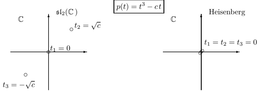
FIGURE 1. Dependence of \mathfrak{g} on the roots of p(t) .
