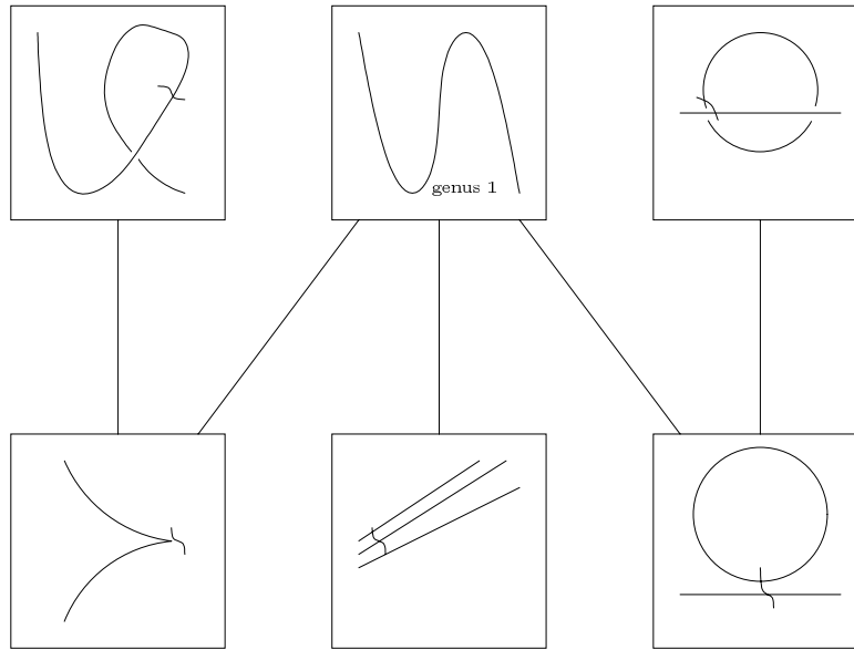
FIGURE 1. Irreducible components and other interesting loci in \overline{\mathcal{M}}_1(\mathbb{P}^2, 3) ; the little squiggle in each panel represents a contracted genus-1 curve.
