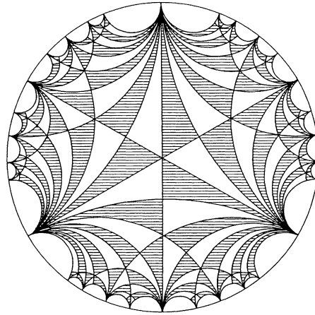
FIGURE 2. Monodromy group SL(2, \mathbf{Z})/\{\pm 1\} in PGL(2, \mathbf{C}) for the hypergeometric differential equation with (a, b, c) = (1/12, 1/12, 2/3) [24, section 0.1].
