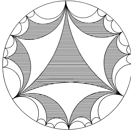
FIGURE 1. Monodromy group \Gamma/\{\pm 1\} in PGL(2, \mathbf{C}) for the hypergeometric differential equation with (a, b, c) = (1/2, 1/2, 1) .
