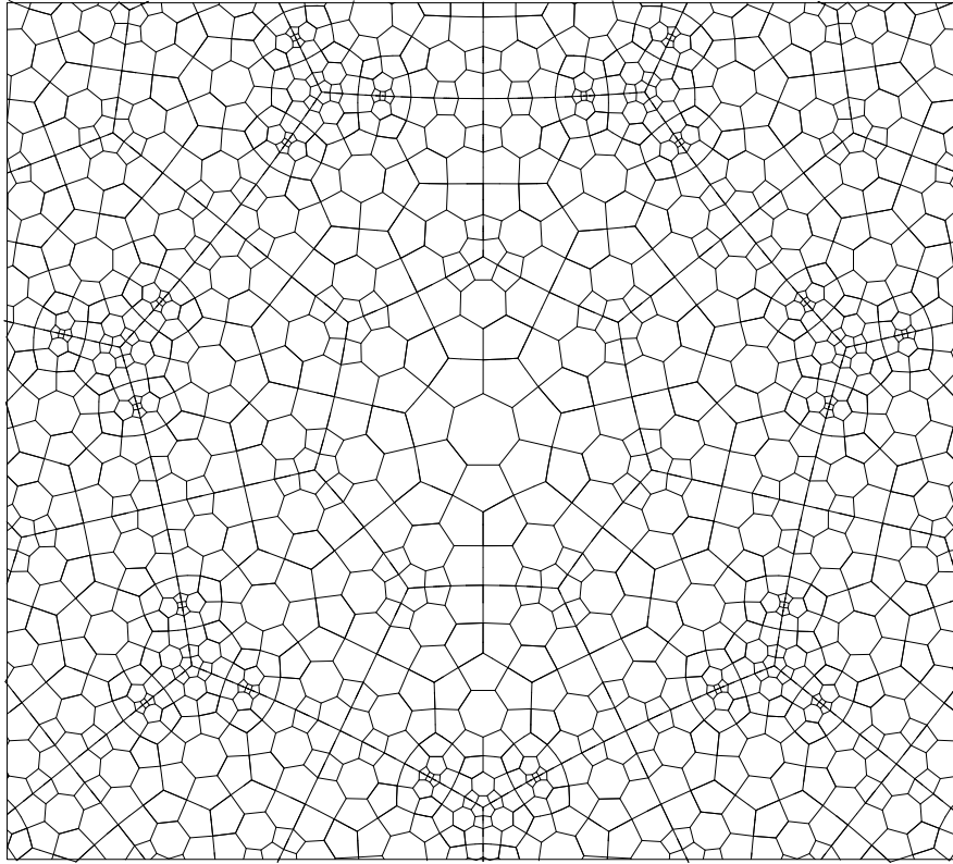
FIGURE 14. A septagonal tiling.
