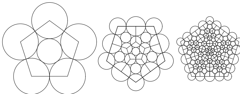
FIGURE 9. The first three stages via packings.
