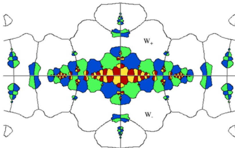
FIGURE 12. Some pieces of the puzzles \mathcal{P}_i , i = 1, 2, 3 .
