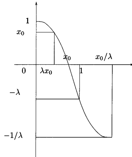
FIGURE 6. The graph of f on \mathbb{R}^+ .
