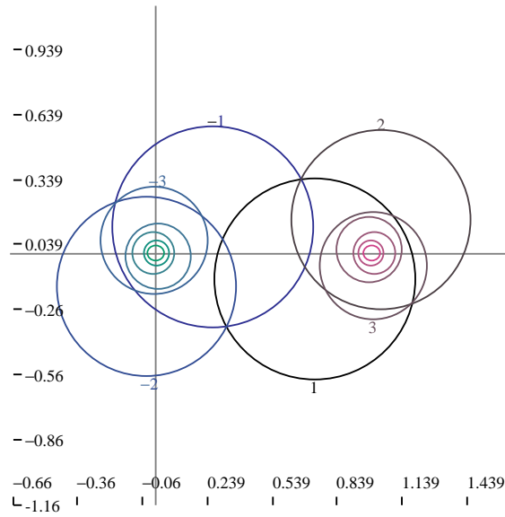
FIGURE 5.11. A four-sided Ford domain
