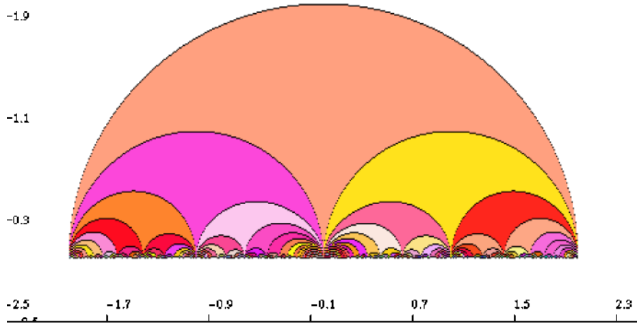
FIGURE 6.1. The decomposition of the trace plane, \rho = \infty
