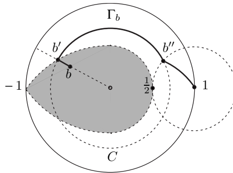
FIGURE 2.1. The region d < 1 - |b| and a slit \Gamma_b
