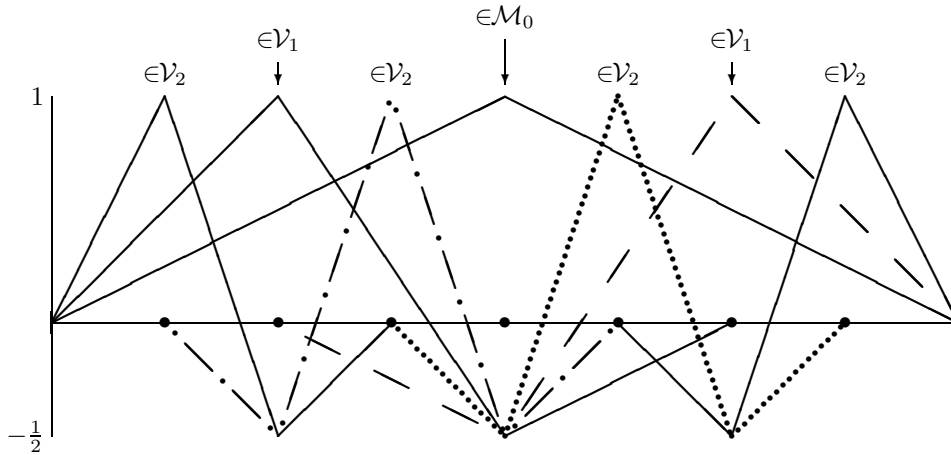
FIGURE 3. Hierarchical basis of \mathcal{M}_2
