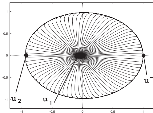
FIGURE 4. Two-dimensional heteroclinic manifold in the u^1u^2 -plane.
