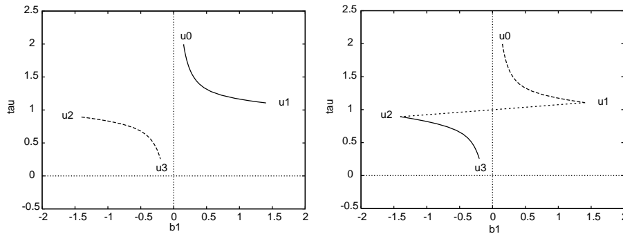
FIGURE 7. Viscous profiles for \omega = 0.01 and \omega = \omega^* in the b^1\tau -plane.
