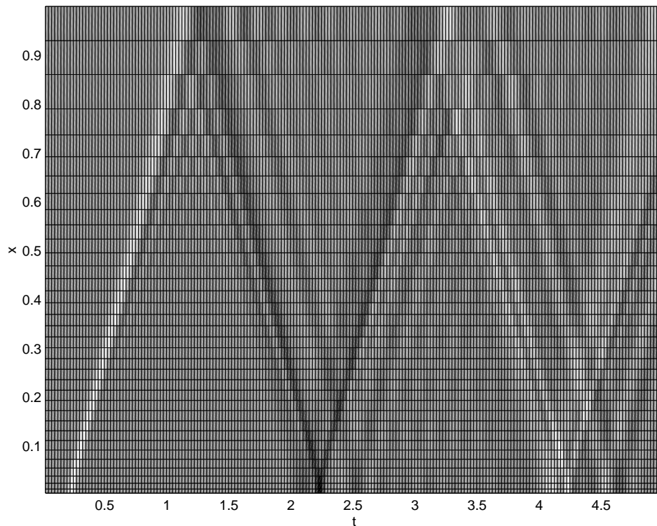
FIGURE 5. The finite-difference solution in x - t coordinates, the optimal grid unbalanced by additional nodes. The numerical dispersion grows monotonically with time.
