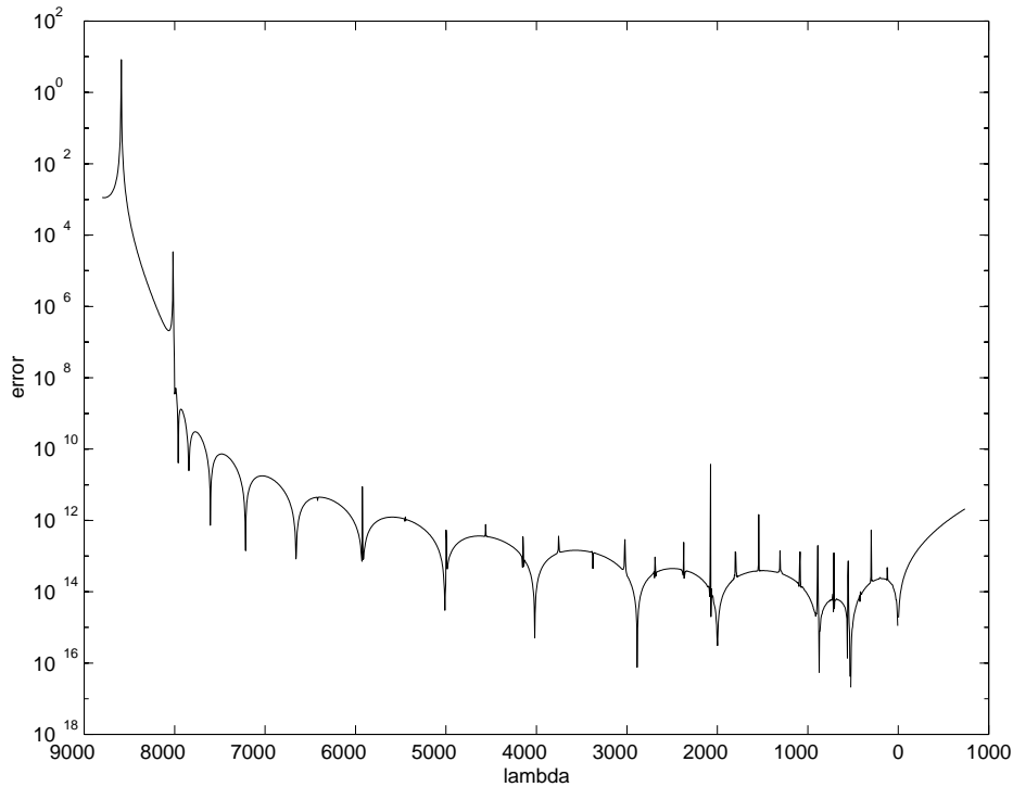
FIGURE 1. The finite-difference impedance error.
