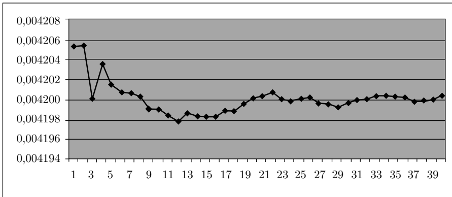
FIGURE 11. The density D(15) of prime numbers with the least primitive root equal to 15
