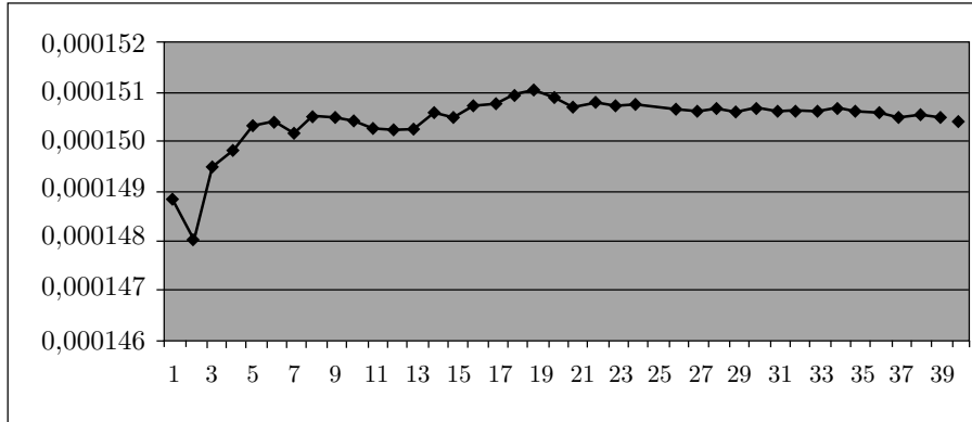
FIGURE 21. The density D(28) of prime numbers with the least primitive root equal to 28
