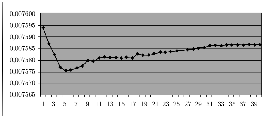
FIGURE 14. The density D(19) of prime numbers with the least primitive root equal to 19
