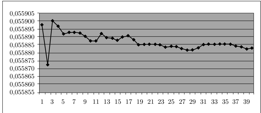
FIGURE 4. The density D(6) of prime numbers with the least primitive root equal to 6
