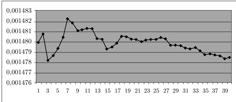
FIGURE 24. The density D(31) of prime numbers with the least primitive root equal to 31
