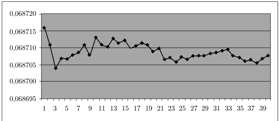
FIGURE 5. The density D(7) of prime numbers with the least primitive root equal to 7
