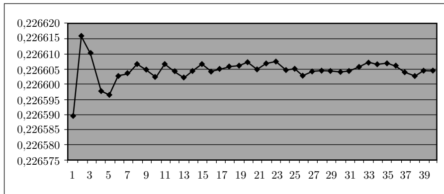
FIGURE 2. The density D(3) of prime numbers with the least primitive root equal to 3
