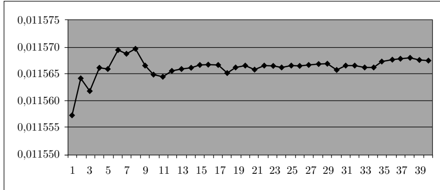
FIGURE 12. The density D(17) of prime numbers with the least primitive root equal to 17
