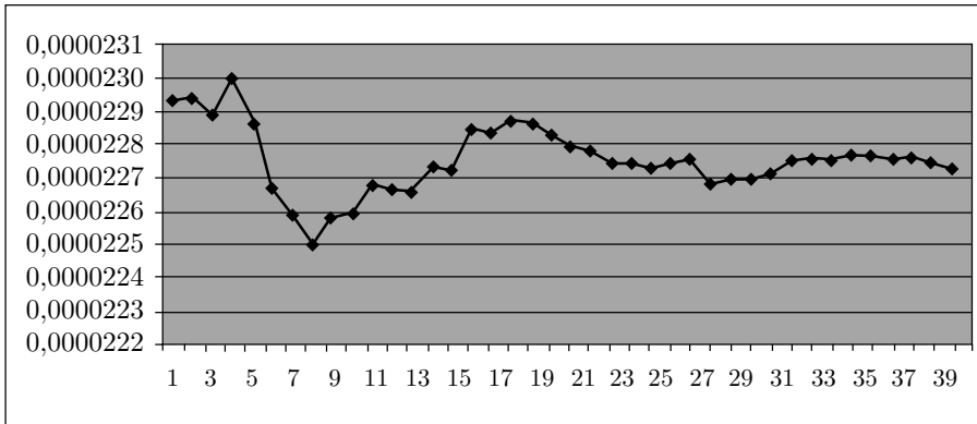
FIGURE 19. The density D(24) of prime numbers with the least primitive root equal to 24
