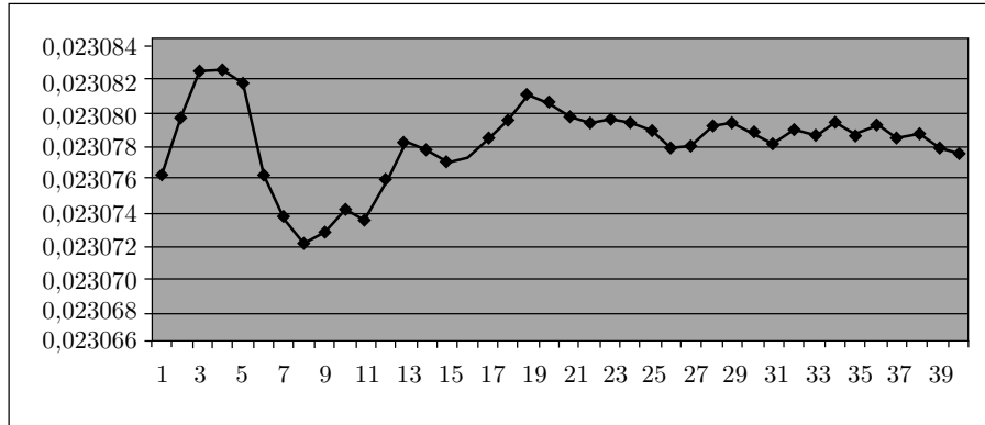
FIGURE 6. The density D(10) of prime numbers with the least primitive root equal to 10
