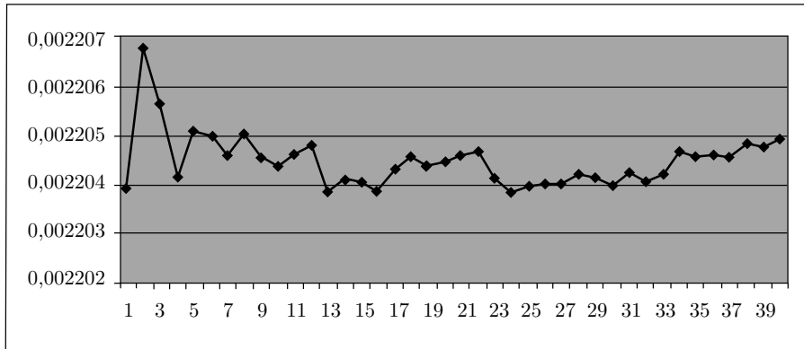
FIGURE 22. The density D(29) of prime numbers with the least primitive root equal to 29
