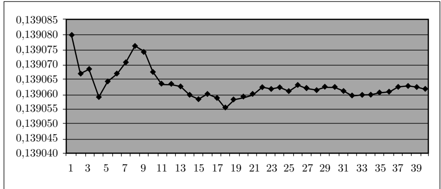
FIGURE 3. The density D(5) of prime numbers with the least primitive root equal to 5
