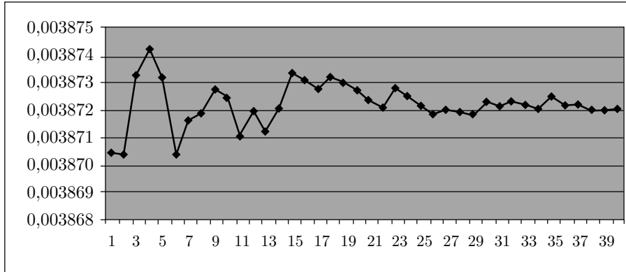
FIGURE 18. The density D(23) of prime numbers with the least primitive root equal to 23
