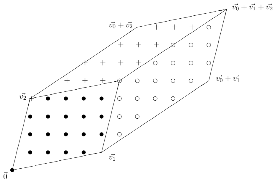
FIGURE 1. The sets V_0 (closed circles), V_1 (open circles) and V_2 (+ signs) formed using \vec{v}_0 = (6, 4) , \vec{v}_1 = (5, 1) and \vec{v}_2 = (1, 4) . Note that |V_0| = \left| \begin{smallmatrix} 5 & 1 \\ 1 & 4 \end{smallmatrix} \right| = 19 , |V_1| = \left| \begin{smallmatrix} 6 & 1 \\ 4 & 4 \end{smallmatrix} \right| = 20 , |V_2| = \left| \begin{smallmatrix} 5 & 6 \\ 1 & 4 \end{smallmatrix} \right| = 14 .
