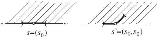
FIGURE 4. Typical neighborhoods of points according to the point is down or up.
