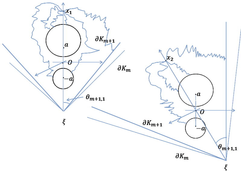
FIG. 1. Solving the direct exterior boundary value problem outside two spheres of unequal radii.
