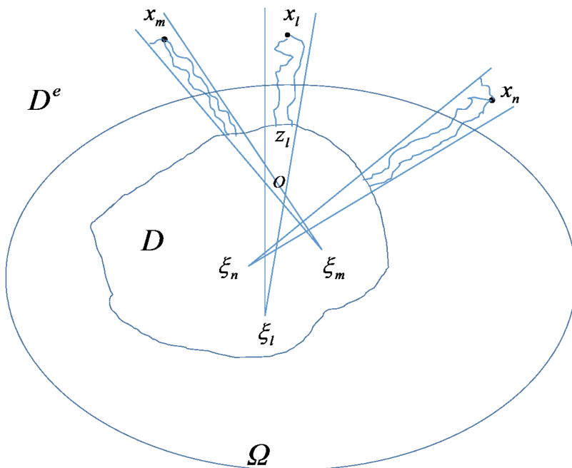
FIG. 3. The narrow cones in the service of the inverse low-frequency scattering problem.
