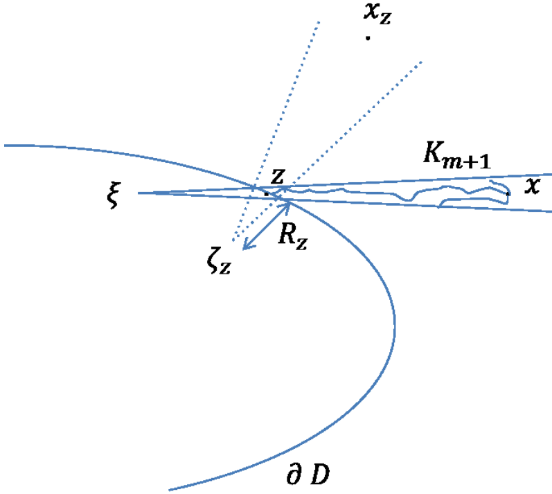
FIG. 4. Every surface point induces a specific cone adapted to the local curvature, which differs from the actual cone of the measurement process.
