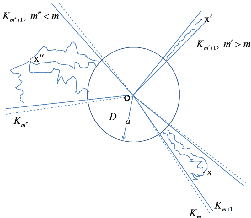
FIG. 2. The strong stochastic solution for the spherical case.
