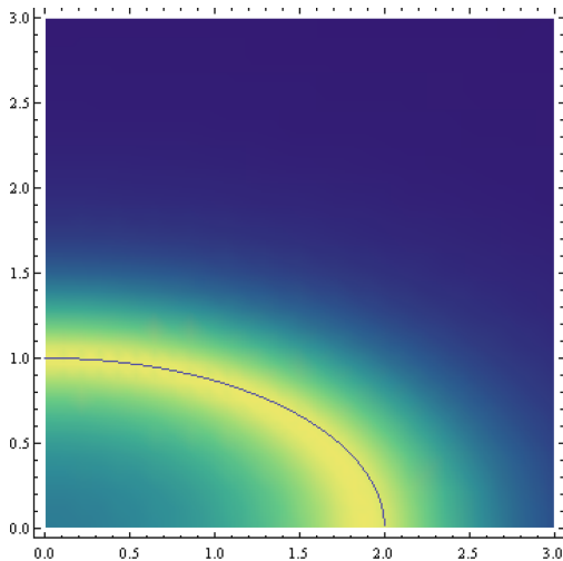
FIG. 5. The reconstruction of the intersection of the ellipsoidal scatterer with the plane x^{(1)} = 0 .
