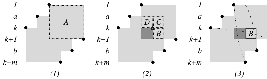
FIGURE 22. We have displayed the case of a < k , but the argument holds for a = k too.
