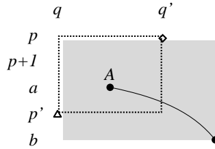
FIGURE 5. \diamond = (p, q') and \Delta = (p', q) .
