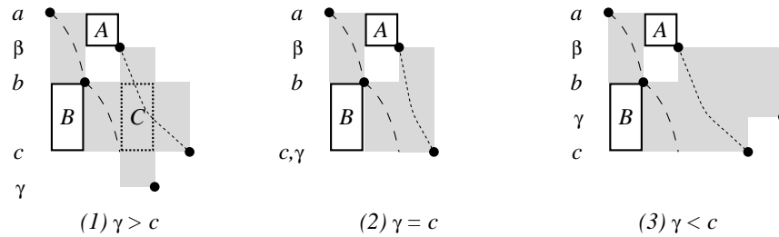
FIGURE 25. We have displayed the case of \beta < b , but the proof of Step 3 also holds for \beta > b .
