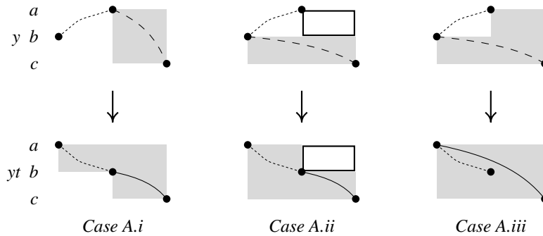
FIGURE 6. Depiction of Case A from Definition 19. The dashed (resp. dotted, solid) arcs represent t' (resp. t , \phi_t(t') ).
