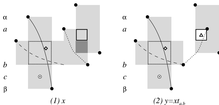
FIGURE 2. We see (among other facts) that d_{x,w}(\diamond) \geq 1 , d_{y,w}(\Delta) = d_{x,w}(\Delta) - 1 \geq 0 , pt_x(c) = pt_w(c) and t_{\alpha,\beta} \in \mathcal{R}(x, w) .
