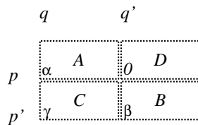
FIGURE 4. We have indicated certain values of d_{x,w} at the lower left corner of each region.
