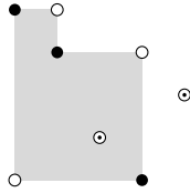
FIGURE 3. In the above configuration, \mathcal{R}(x, w) = \{t_{1,2}, t_{2,4}, t_{2,5}, t_{4,5}\} .
