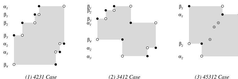
FIGURE 1. Possible differences between permutation matrices for x \in \text{maxsing}(X_w) as described in Theorem 1. \circ 's denote 1's in \text{mat}(w) ; \bullet 's denote 1's in \text{mat}(x) .
