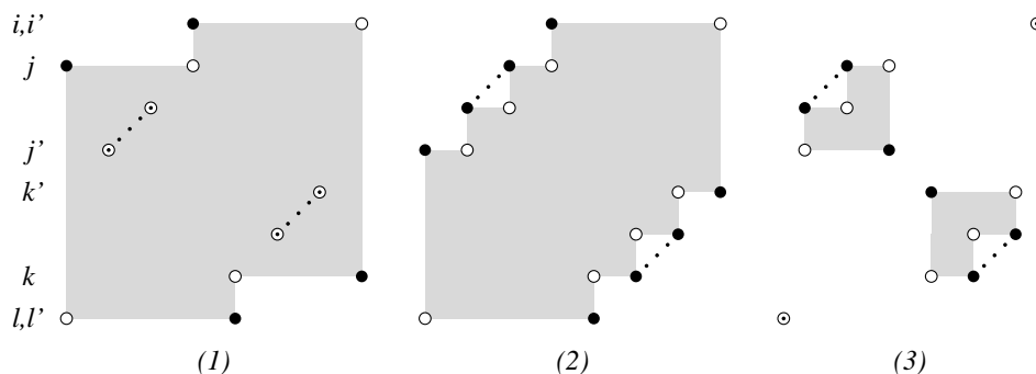
FIGURE 31. (1) \underline{w}, w ; (2) x, w ; (3) \hat{x}, w .
