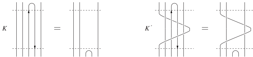
FIGURE 8. Reducing the number k_\uparrow of negative strands
