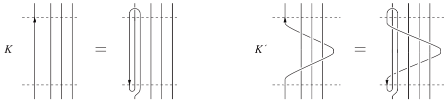
FIGURE 7. Transforming a negative Kirby move into a positive one
