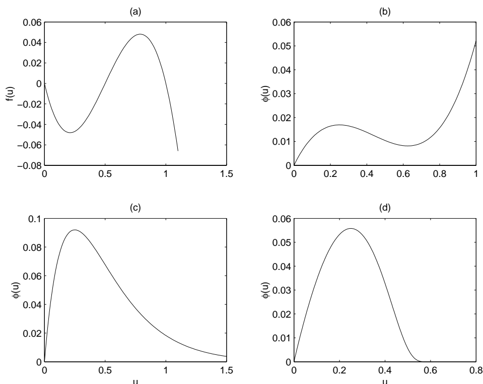
FIGURE 1. (a) f(u) = u(u - a)(b - u) , with a = 1/2 and b = 1 ; (b) \phi(u) = (u^3/3 - (\alpha + \beta)u^2/2 + \alpha\beta u) , with \alpha = 1/4 and \beta = 5/8 ; (c) \phi(u) = ue^{-\frac{u}{\alpha}} , with \alpha = 1/4 ; (d) \phi(u) = u \exp \frac{(\beta - \alpha)^2}{\alpha(u - \beta)} if 0 \leq u < \beta and \phi(u) = 0 if u \geq \beta , with \alpha = 1/4 and \beta = 5/8 .
