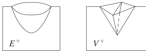
FIGURE 14. Types of critical points in \mathcal{C}^1
