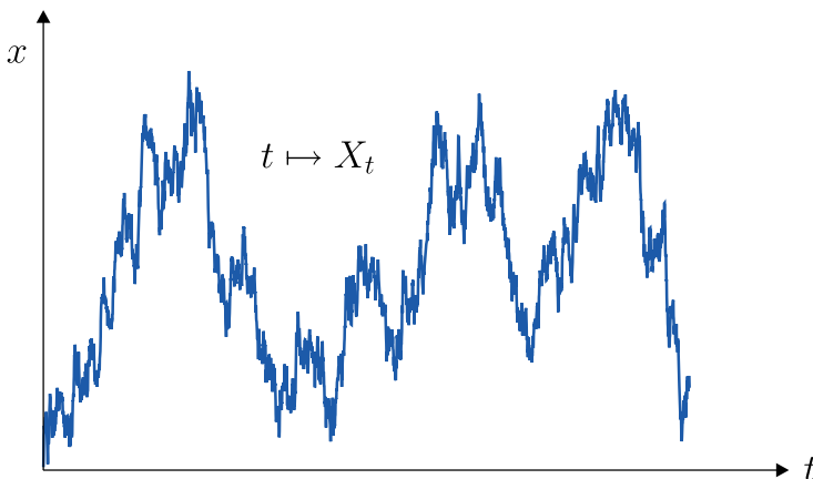
FIGURE 1. Distance to the origin of a Brownian particle whose simulated motion takes place either in a two-dimensional plane or in three-dimensional space.
