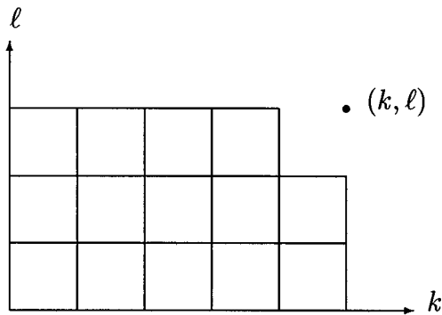
FIGURE 2. Dependency graph
