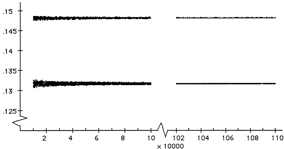
FIGURE 4.1. A point (q, f(q)) represents a value of q in [10000, 100000] or [1020000, 1100000] together with the observed proportion, f(q) , of M \in I_q(4) whose 3-Sylow subgroup of \mathcal{Cl}(\mathcal{O}_M) is isomorphic to C_3 . The upper and lower ‘lines’ correspond to q \not\equiv 1 \pmod{3} and q \equiv 1 \pmod{3} , respectively.
