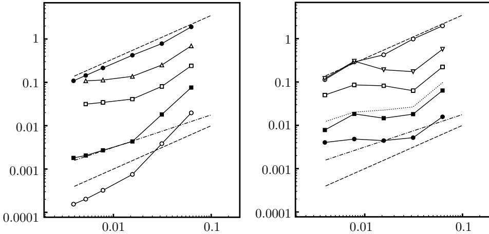
FIGURE 1. Relative L^2 -error against mesh-size, left unperturbed data, right with 1% relative noise. Reference lines are the same in both plots and of orders, dashed lines \approx O(h) with different constants, dash dot \approx O(h^{\frac{3}{4}}) and dotted C_1 \|e\|_{\Omega}^{0.3} (r_1 + r_2)^{0.7} + 10h^2 .
