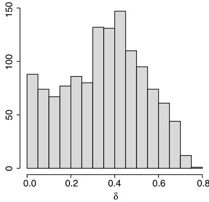
FIGURE 1. Distribution of non-cyclotomic factors F(X) of polynomials from \mathcal{B}_{\leq 9} such that F(X) \in \mathcal{L}(\mathbb{Z}[X]) .
