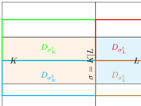
FIGURE 4. Full grid velocity interpolate.
