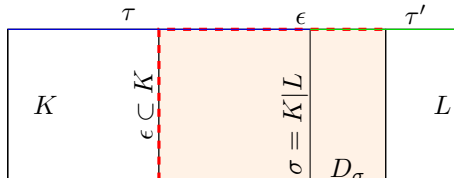
FIGURE 2. Notation for the dual fluxes of the first component of the velocity.
