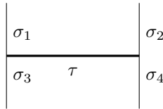
FIGURE 5. Neighboring faces of \tau
