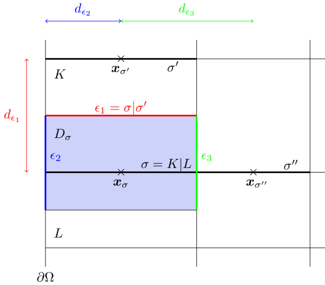
FIGURE 1. Notation for control volumes and dual cells (for the second component of the velocity).
