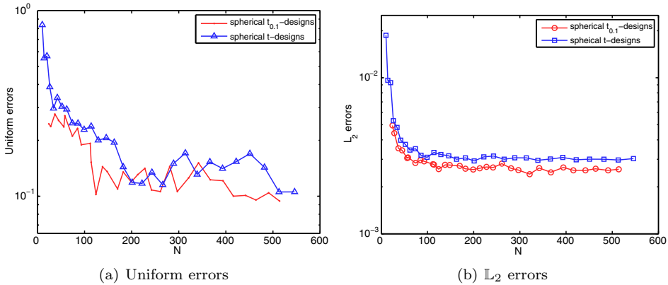
FIGURE 5.2. Errors for approximating Franke function with different scales of point sets
