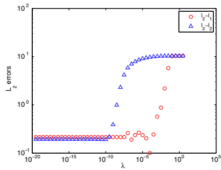
(b) L_2 errors with different \lambda for \delta = 0.1
