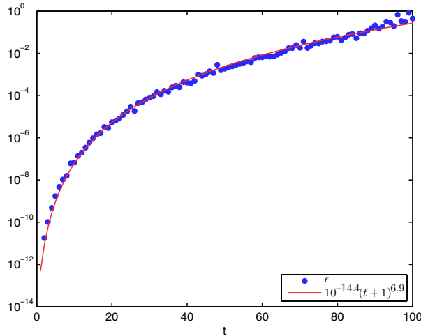
FIGURE 3.1. \epsilon computed by (3.19) for t = 2, \dots, 100
