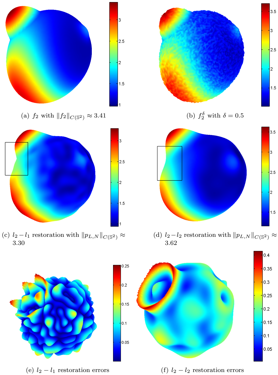
FIGURE 5.3. Restoration of f_2 using spherical 37_{0.1} -design with models (5.2) and (5.3)
