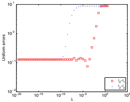
(a) Uniform errors with different \lambda for \delta = 0.1
