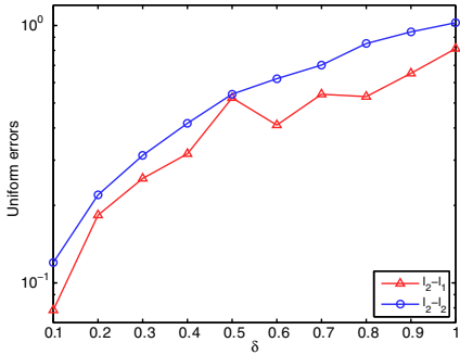
(c) Minimal uniform errors with different noise scales \delta
