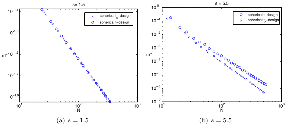
FIGURE 4.1. Worst-case errors for spherical t_{0,1} -designs and spherical t -designs
