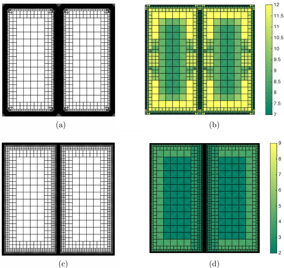
FIGURE 11. Ginzburg-Landau equation. Computational meshes. Left: h -refinement; right: hp -refinement. (a) and (b) \epsilon = 10^{-3} ; (c) and (d) \epsilon = 10^{-6} .
