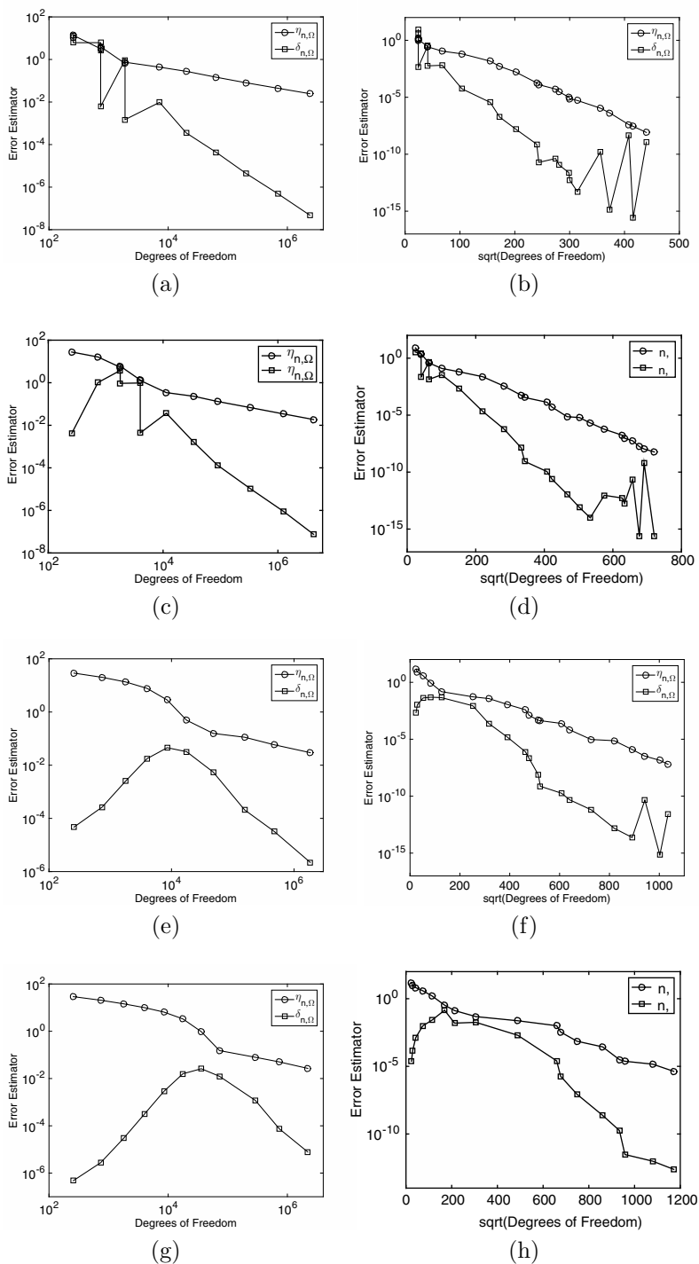
FIGURE 9. Ginzburg-Landau equation. Individual error indicators \eta_{n,\Omega} and \delta_{n,\Omega} . Left: h -refinement; right: hp -refinement. (a) and (b) \epsilon = 10^{-3} ; (c) and (d) \epsilon = 10^{-4} ; (e) and (f) \epsilon = 10^{-5} ; (g) and (h) \epsilon = 10^{-6} .
