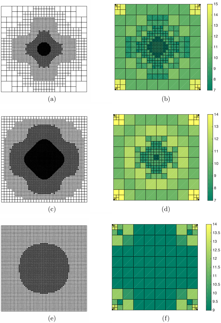
FIGURE 6. Bratu Problem. Computational meshes. Left: h -refinement; right: hp -refinement. (a) and (b) Upper solution computed with \epsilon = 1 ; (c) and (d) Upper solution computed with \epsilon = 0.5 . (e) and (f) Critical solution.
