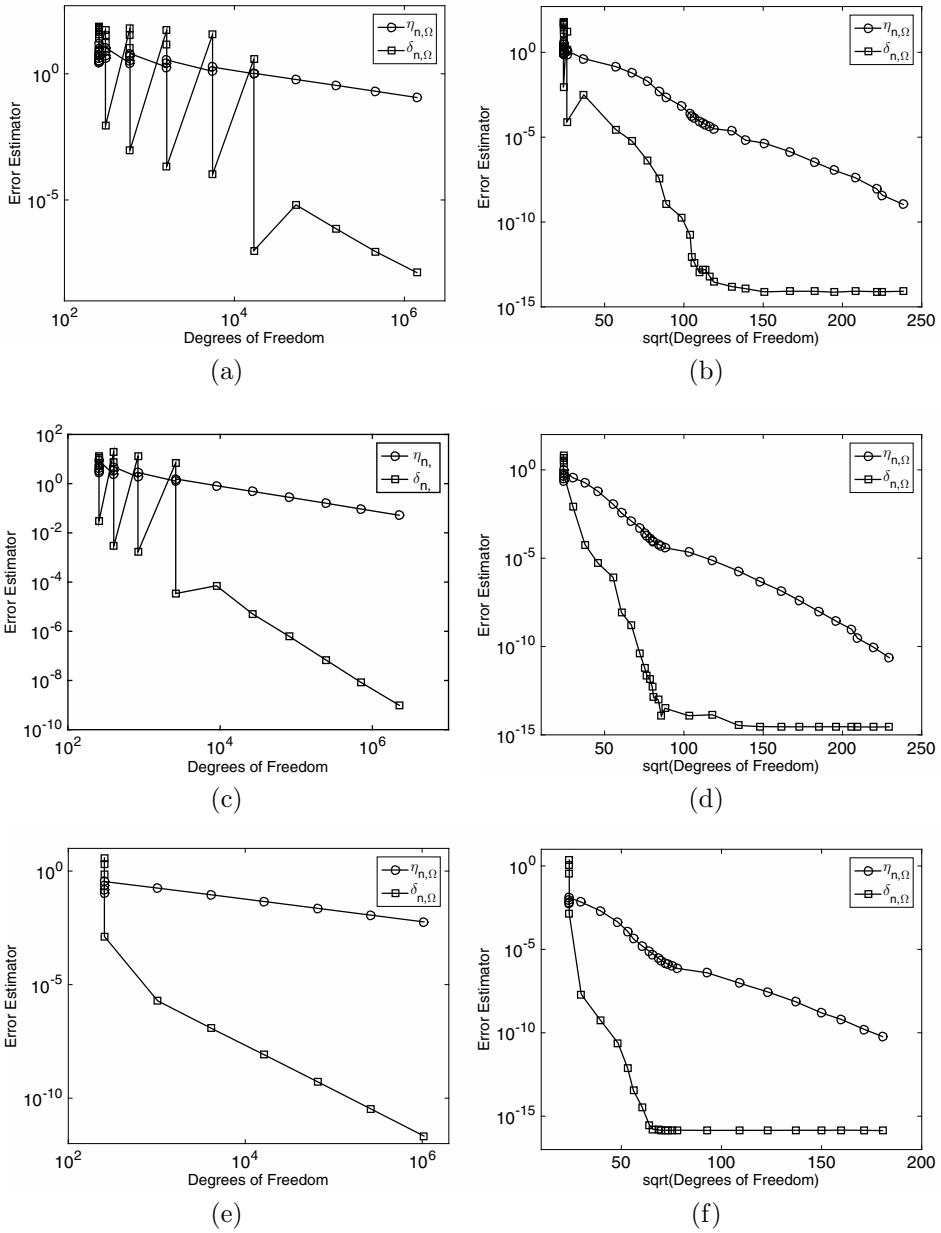
FIGURE 5. Bratu Problem. Individual error indicators \eta_{n,\Omega} and \delta_{n,\Omega} . Left: h -refinement; right: hp -refinement. (a) and (b) \epsilon = 1 (upper solution); (c) and (d) \epsilon = 1/2 (upper solution); (e) and (f) \epsilon = 1/2 (lower solution).
