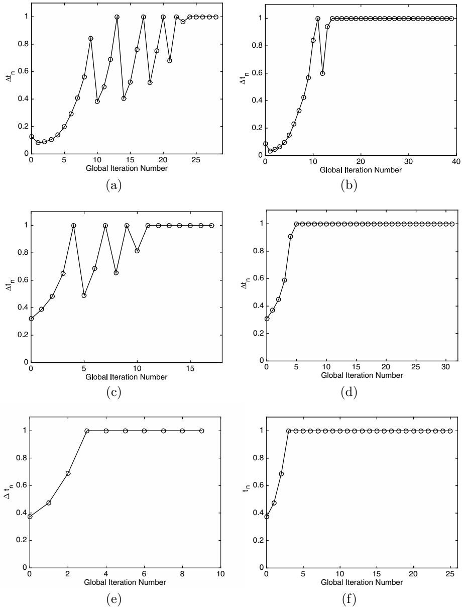
FIGURE 4. Bratu Problem. Damping parameter \Delta t_n . Left: h -refinement; right: hp -refinement. (a) and (b) \epsilon = 1 (upper solution); (c) and (d) \epsilon = 1/2 (upper solution); (e) and (f) \epsilon = 1/2 (lower solution).
