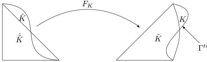
FIGURE 8. A curved element K \in \mathcal{T}^{tr} and the related q -degree parametric element \hat{K} as the mapping of the respective reference elements \hat{\hat{K}} and \hat{K} .
