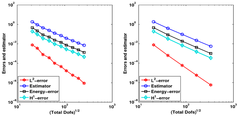
FIGURE 9. Example 1. Convergence of the estimator and errors for quadratic mapping and p = 2 : adaptive (left) and uniform (right) refinements.
