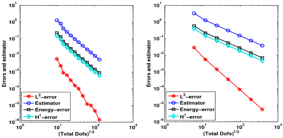
(b) p = 2
