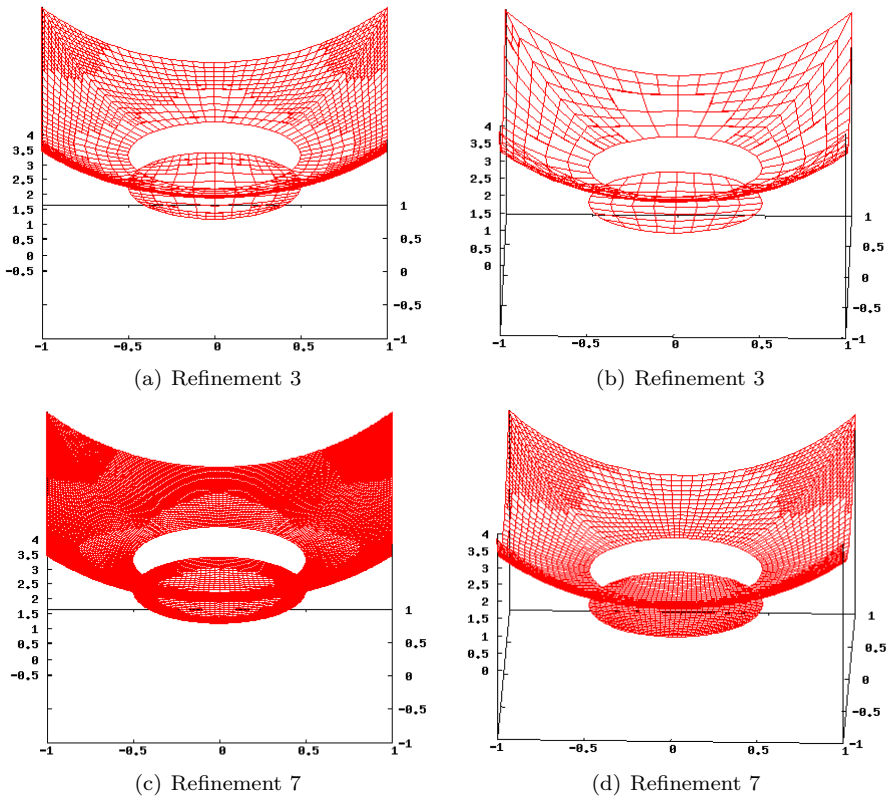
FIGURE 10. Example 1. Meshes produced by the adaptive algorithm with quadratic mapping, for p = 1 (left) and p = 2 (right).
