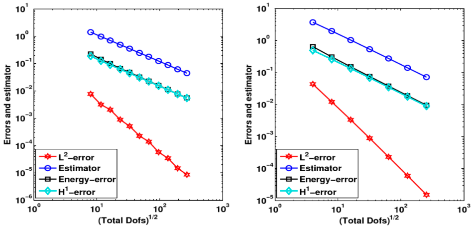
(a) p = 1
