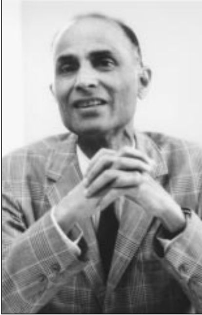
Harish-Chandra.
