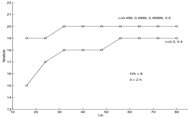
FIGURE 1. Elasticity problem with P_1(h) - P_1(2h) finite elements: iteration counts for GMRES with overlapping additive Schwarz preconditioner \mathcal{B}^{-1}
