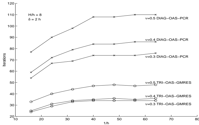
FIGURE 2. Elasticity problem with P_1(h) - P_1(2h) finite elements: iteration counts for PCR with block-diagonal (DIAG-OAS-PCR) and GMRES with block-triangular (TRI-OAS-GMRES) preconditioners using the overlapping additive Schwarz preconditioner as block solver.
