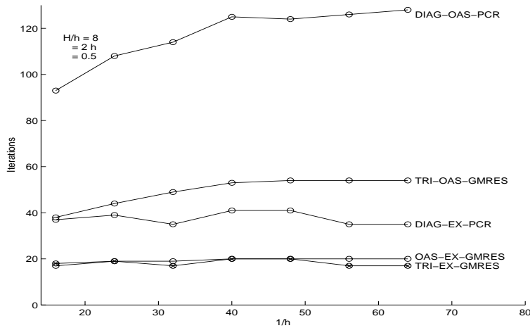
FIGURE 3. Elasticity problem with P_1(h) - P_1(2h) finite elements: iteration counts for different preconditioners; OAS-EX-GMRES=GMRES with overlapping additive Schwarz and exact subdomain solvers, DIAG-OAS-PCR=PCR with block-diagonal preconditioner and overlapping additive Schwarz as block solvers, TRI-OAS-GMRES=GMRES with block-triangular preconditioner and overlapping additive Schwarz as subdomain solvers, DIAG-EX-PCR=PCR with block-diagonal preconditioner and exact block solvers, and TRI-EX-GMRES=GMRES with block-triangular preconditioner and exact block solvers.
