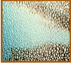
Figure 1. Carbon dioxide is injected in a “mini-reservoir” in a laboratory. Rock grains are visible as white spheres. Brown oil is seen in the pores of the rock, but where the carbon dioxide flows, the oil is no longer in the pores: it has been produced and the rock has been swept clean. This is what oil engineers hope to achieve below the subsurface also. The only possible way to assess this process is through mathematical modeling.
