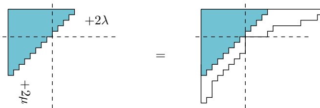
FIGURE 1. A 2-separated partition \tau_\mu^\lambda (see Definition 1.6)
