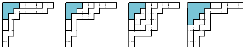
FIGURE 2. Examples of partitions which label 2-height 0 characters for \mathfrak{S}_{28} and \mathfrak{S}_{36} (and therefore label constituents of Saxl’s tensor square by Theorem B). There are 672 and 1417 such characters for these groups, respectively. A combinatorial construction of all such partitions (for arbitrary n \in \mathbb{N} ) is given in Subsection 1.4.
