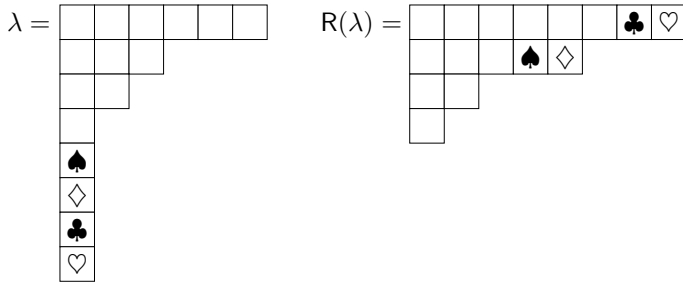
FIGURE 5. The partition \lambda = \tau_{(12)}^{(1)}(4) , its 2-regularisation R(\lambda)
