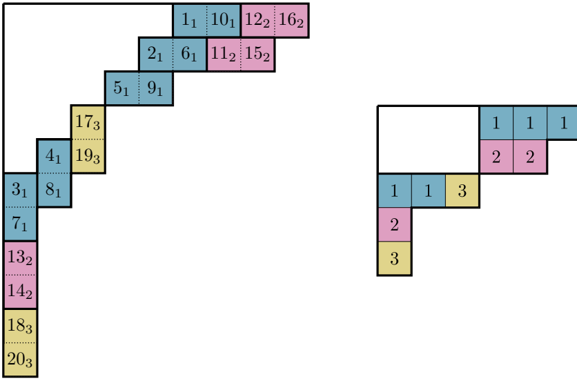
FIGURE 7. A (3^2, 2, 1^2) -decorated standard tableau of shape \tau_{(3,1,1)}^{(2,2,1)} \setminus \tau and the corresponding element of \text{SStd}((3, 2) \cup (3, 1, 1), (5, 3, 2)) . The associated sequence of partitions (as in equation (4.6)) is \tau \subset \tau_{(2)}^{(1^3)} \subset \tau_{(2,1)}^{(2^2,1)} \subset \tau_{(3,1^2)}^{(2^2,1)} .
