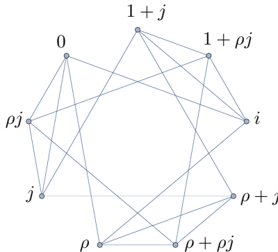
FIGURE 7. The 1-skeleton of the 3-3 duoprism
