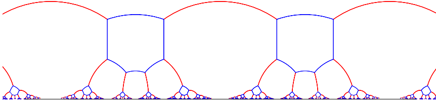
FIGURE 12. Ocean of the Hermitian form f(u, v) = \text{tr}(\bar{u}v) over \mathbb{Z}[\frac{1+i\sqrt{3}}{2}]
