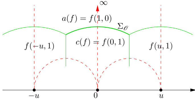
FIGURE 11. Values of F on Ford-Voronoi cells meeting \Sigma_{\mathcal{O}}
