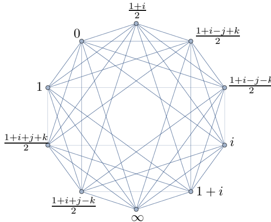
FIGURE 6. Pattern of intersections into 4-dimensional cells of Ford-Voronoi cells centered at \{\infty, 0, 1, i, i+1, \frac{1+i+j+k}{2}, \frac{1+i}{2}\}
