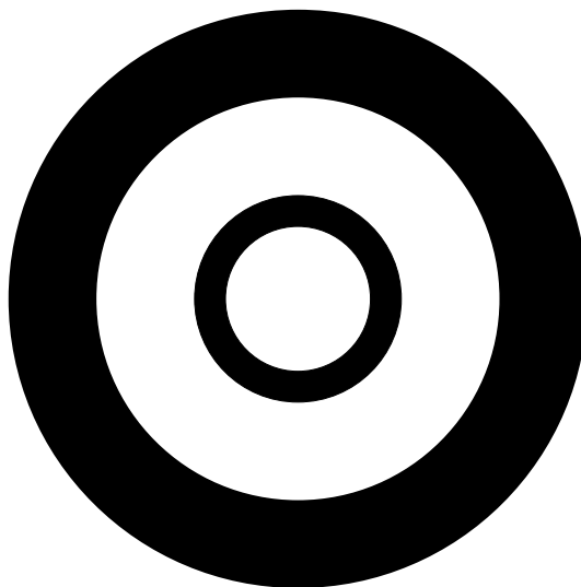
FIGURE 10. A schematic for Lemma 12.1. W_k^n and W_{k-1}^n belong to the same covering \mathcal{C}_m , and W_{k-1}^n is contained inside of the bounded complementary component of W_k^n . When R is large and k \geq 1 , both components are approximately round and the diameter of W_{k-1}^n is controlled in terms of the diameter of W_k^n .
