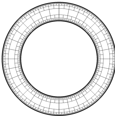
FIGURE 12. An illustration of a Whitney-type decomposition of the annulus described in Lemma 14.4
