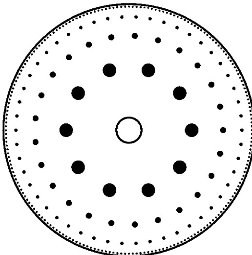
FIGURE 8. A schematic for Lemma 12.2. W_k^n belongs to the covering \mathcal{C}_m and is the annulus bounded by the innermost and outermost boundary curves. The filled components correspond to elements \widehat{W}_{k+q-1}^{n+q} of \widehat{\mathcal{C}}_{m+1} for q = 1, 2, 3, 4 . Lemma 12.2 says when R is large enough and k \geq 1 , the \alpha -sum of these components in \widehat{\mathcal{C}}_{m+1} can be controlled in terms of \text{diam}(W_k^n)^\alpha .
