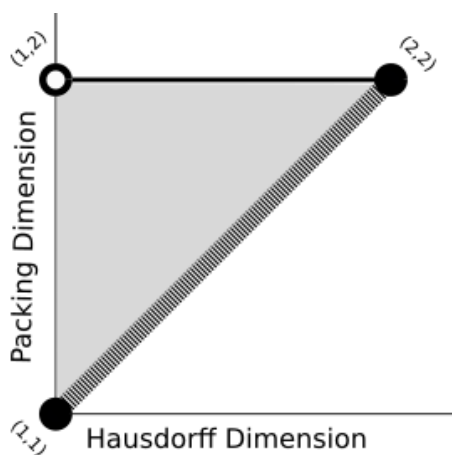
FIGURE 1. A graphic showing the possible and attained Hausdorff and packing dimension pairs for transcendental entire functions. All possible pairs are shaded in light gray, and all attained values are colored black. The point (2, 2) is attained by families of the exponential and sine functions. The upper segment is due to the work of Stallard, and the point (1, 1) is due to Bishop. Our contribution uses enlarged, dashed lines, to emphasize that a dense set of dimensions is attained very close but perhaps not on the diagonal.
