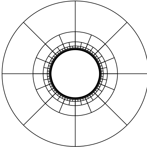
FIGURE 4. The Whitney-type decomposition in Example 4.4 for the case N = 2 . In this picture the “squares” form a Whitney-type decomposition for a neighborhood of \overline{B(0,1)} . Each square in the picture has the property z^2 maps a square in one ring of squares to one in the next ring, normalized so that one of the squares in each ring has a radial segment on the real axis.
