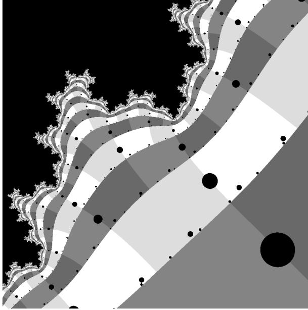
FIGURE 9. A schematic for Lemma 13.1. We see a portion of B_f , and we see annular regions representing the innermost and outermost boundaries of Fatou components \Omega_k for k \leq 0 . The complimentary components of \Omega_k contained in \Omega_k^A are filled in and correspond to the elements in \mathcal{V}_k . Inside each annular region, we have depicted the pieces of \Omega_k that make up the collection \mathcal{Q} , which is a Whitney-type decomposition of a neighborhood of the unbounded complementary component of J_f .
