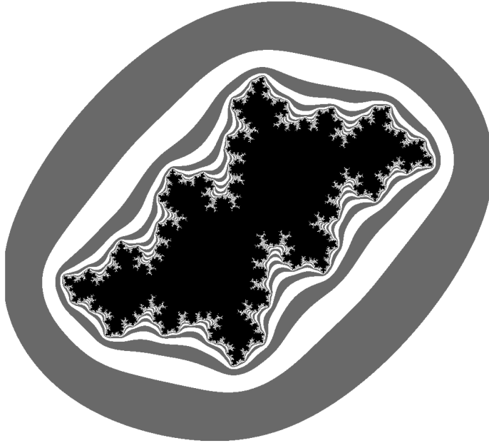
FIGURE 3. A schematic for a sequence of wiggly Fatou components, alternating between gray and white. The holes have been omitted to emphasize the wiggly shape of the inner and outer boundaries. These boundary components approximate level lines for the Green's function of the complement of the closure of the basin of attraction, and they surround and accumulate on the basin's fractal boundary.
