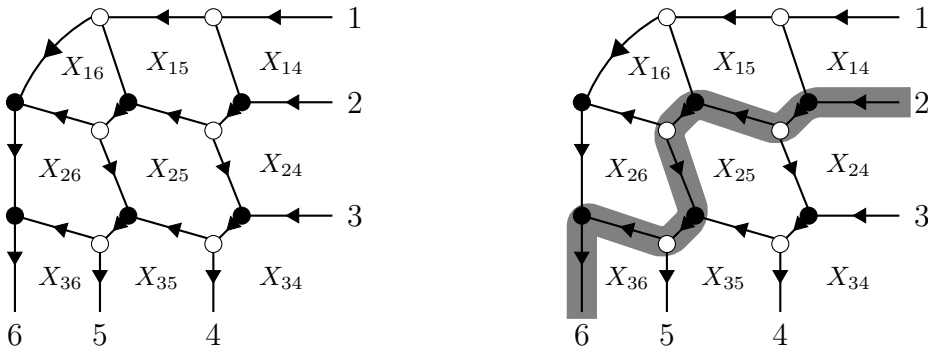
FIGURE 1. \text{Web}_{k,n} for k = 3 and n = 6 . If w is the path on the right-hand side, then \text{wt}(w) = x_{25}x_{24}x_{36}x_{35}x_{34} and \text{Wt}(w) = X_{25} + X_{24} + X_{36} + X_{35} + X_{34} .
