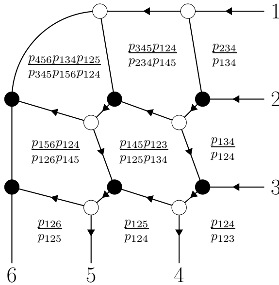
FIGURE 2. Inverting the map.
