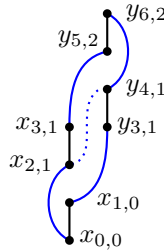
FIGURE 1.4. We depict a singly-generated free \mathcal{A}^{\mathbb{R}}(1) -module, where each \bullet represents a M_2^{\mathbb{R}} -generator. The black and blue lines represent the action of motivic Sq^1 and Sq^2 , respectively. A dotted line represents that the action hits the \tau -multiple of the given M_2^{\mathbb{R}} -generator.
