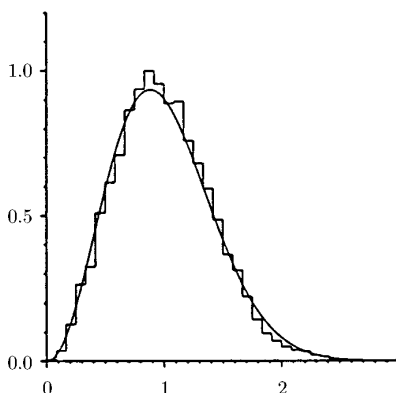
FIGURE 4. Nearest neighbor spacings distribution for the L -function associated to E: y^2 + y = x^3 - x, N = 5374 .
