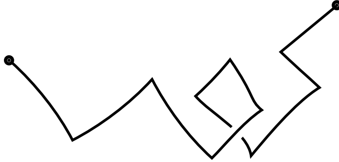
FIGURE 11. A us-path alternates between unstable and stable arcs. It is potentially like a corkscrew.
