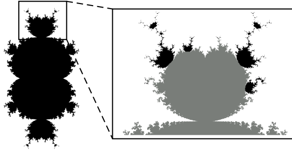
FIGURE 2. The figure on the left shows the connectedness locus \mathcal{M}_3 . The figure on the right is an enlargement of a primary limb in \mathcal{M}_3 . The dark regions in the right box show some of the secondary limbs.
