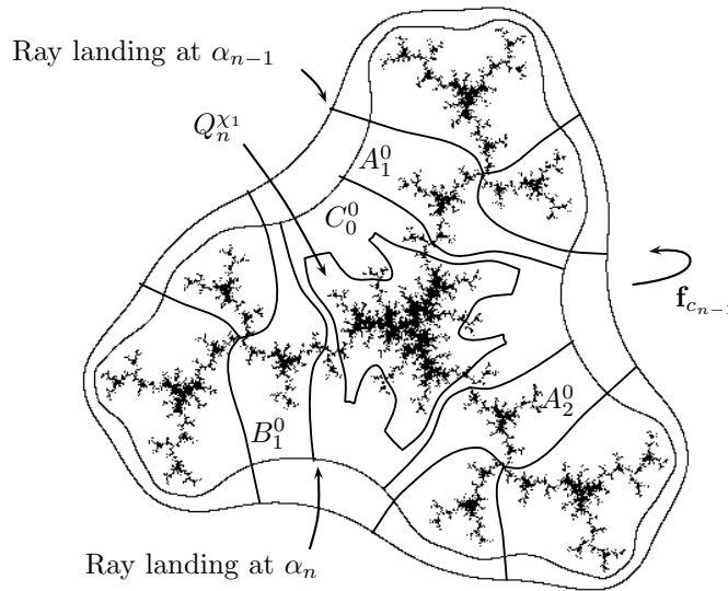
FIGURE 6. The figure shows an infinitely renormalizable Julia set. The first renormalization is of satellite type and the second one is of primitive type. The puzzle piece Q_n^X1 at the center is the first puzzle piece in the favorite nest.
