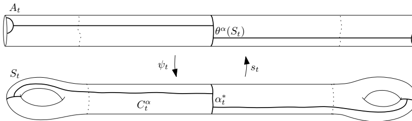
FIGURE 4. The covering annulus A_t \rightarrow S_t corresponding to \alpha_t .
