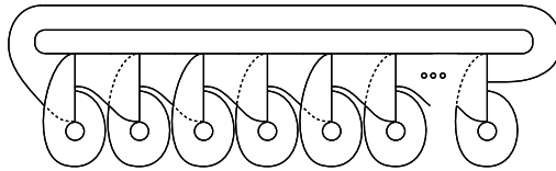
FIGURE 3. The template \mathcal{W}_q is a q -fold cover of \mathcal{V} .
