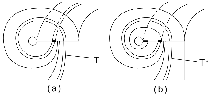
FIGURE 4. (a) A closeup of the top ear of \mathcal{V} and a subtemplate \mathcal{T} ; (b) appending an ear to \mathcal{T} yields \mathcal{T}^+ .
