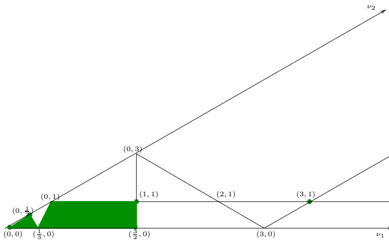
FIGURE 1. Spherical unitary dual for \mathbb{H}(G_2, (3, 1))
