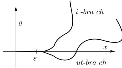
FIGURE 1. A singular curve with a needle.
