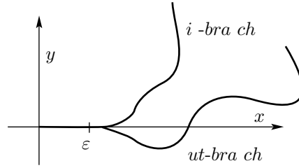
FIGURE 1. A singular curve with a needle.
