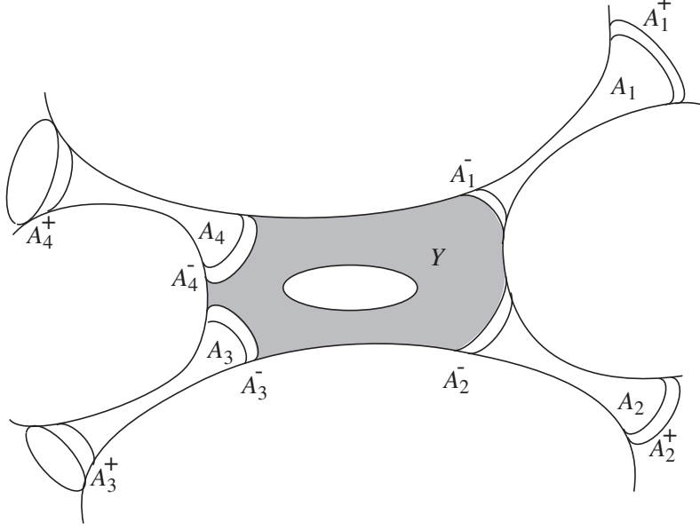
FIGURE 4. One thick piece Y with its adjacent annuli A_1, \dots, A_n . (Some annuli A_i might be adjacent to Y at both ends.)
