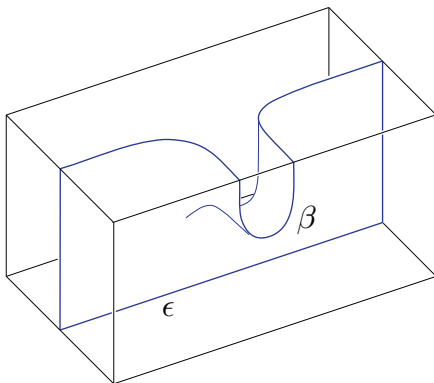
FIGURE 8.13. The rectangular solid N contains D' \cap N .
