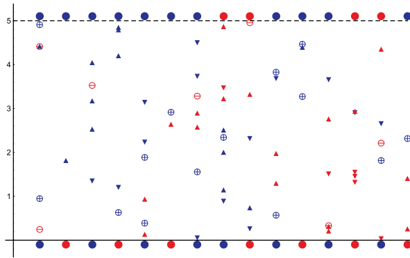
FIGURE 4. Heat-bath dynamics for the 1D Ising model, marking oblivious updates by \oplus and \ominus and non-oblivious updates by \blacktriangle and \blacktriangledown to denote \sigma(i) \mapsto \sigma(i-1) \wedge \sigma(i+1) and \sigma(i) \mapsto \sigma(i-1) \vee \sigma(i+1) . (Color available online.)
