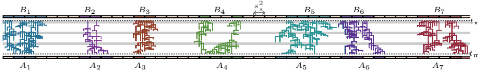
FIGURE 8. Components \mathcal{A} = \{A_i\} and \mathcal{B} = \{B_i\} corresponding to \{\Upsilon_i\} . Each \Upsilon_i joins vertices of \Upsilon via history intersection ; \Upsilon_4 and \Upsilon_7 also join vertices via final proximity and initial proximity , resp. (Color available online.)
