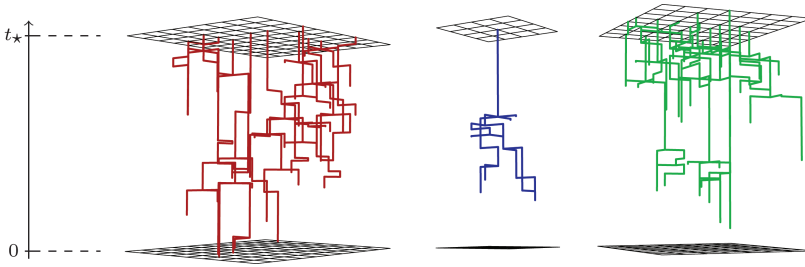
FIGURE 6. Red, blue, and green information percolation clusters as per Definition 2.3. ( Color available online. )
