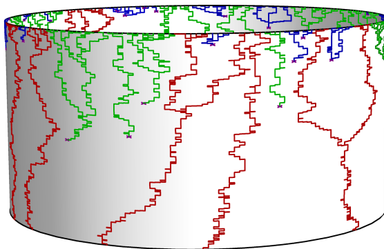
FIGURE 3. Information percolation clusters in Glauber dynamics for the 1D Ising model: red (reaching time zero), blue (dying out quickly), and green clusters on n = 256 sites. ( Color available online. )
