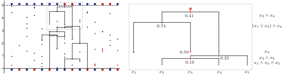
FIGURE 5. Update support for heat-bath dynamics for the 1D Ising model at \beta = 0.4 ( \theta \approx 0.34 ); the zoomed-in part shows the update history with the root spin as a deterministic function of the leaves. (Color available online.)
