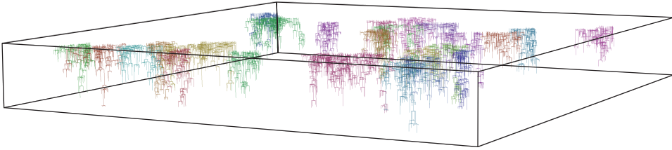
FIGURE 1. Information percolation clusters for the two-dimensional (2D) stochastic Ising model: showing the largest 25 clusters on a \{1, \dots, 200\}^2 \times [0, 20] space-time slab. ( Color available online. )
