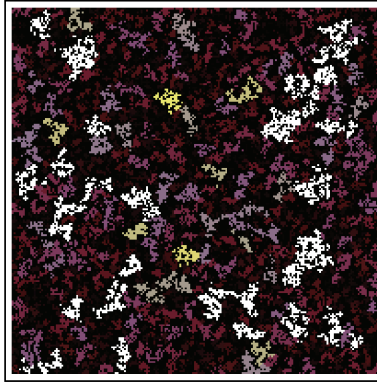
FIGURE 2. Top view of information percolation clusters for the 2D stochastic Ising model: sites of a 200 \times 200 square color-coded by their cluster size (increasing from red to white). ( Color available online. )
