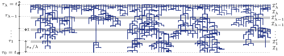
FIGURE 7. Regular phases ( \mathcal{I}_k ) and deferred phases ( \mathcal{I}'_k ) of the update history in the range t > t_m : no vertices are removed from the support along the deferred phases (marked by shaded regions). (Color available online.)
