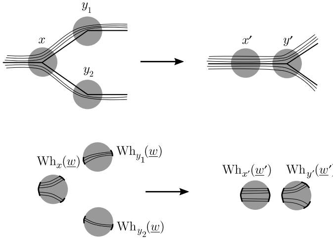
FIGURE 2. The effect of a fold on Whitehead graphs. Note that Wh_{x'}(\underline{w}') is obtained by wedging Wh_x(\underline{w}) , and Wh_{y'}(\underline{w}') is obtained by wedging Wh_{y_1}(\underline{w}) \sqcup Wh_{y_2}(\underline{w}) .
