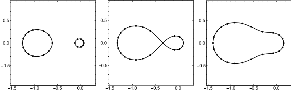
FIGURE 6. The pictures represent the roots of the equation w^N(w + 1)^{L-N} = z^L and the contours |w^N(w + 1)^{L-N}| = |z|^L with N = 8, L = 24 for three different values of z . The value of |z| increases from the left picture to the right picture. The middle picture is when z = \rho^\rho(1 - \rho)^{1-\rho} , where \rho = N/L = 1/3 .
