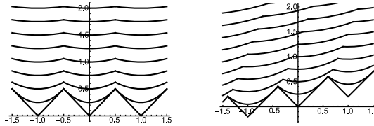
FIGURE 2. The pictures represent the limiting height function at times t = 0.5nL for n = 0, 1, 2, \dots . The left picture is when \rho = 1/2 and the right picture is when \rho = 2/5 . Both the horizontal axis (location) and the vertical axis (height) are scaled down by L .
