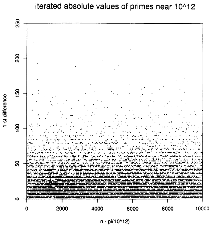
FIGURE 1. Differences d_1(n) for 10^4 primes near 10^{12}
