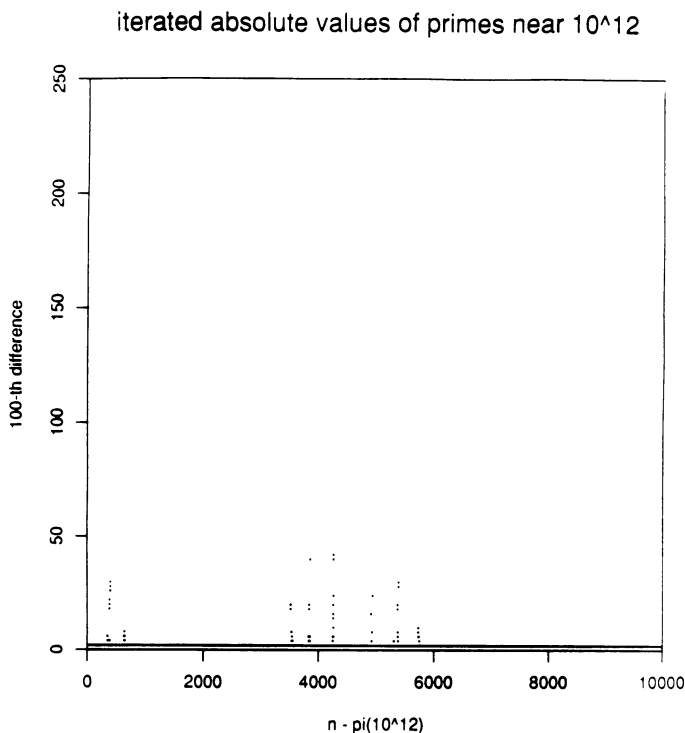
FIGURE 3. Differences d_{100}(n) for 10^4 primes near 10^{12}
