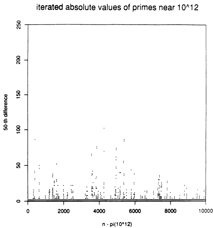
FIGURE 2. Differences d_{50}(n) for 10^4 primes near 10^{12}
