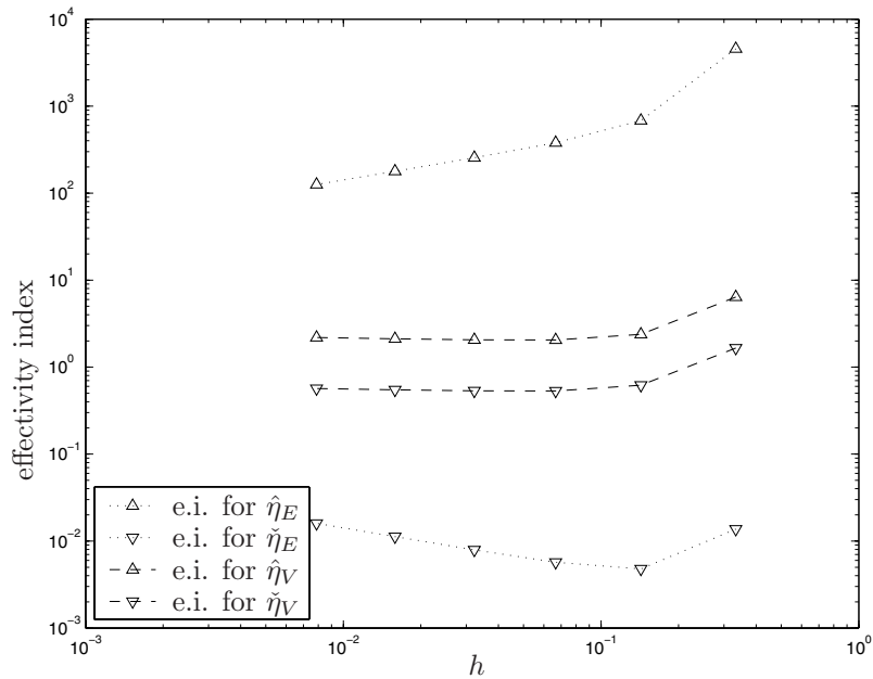
FIGURE 6. Effectivity indexes for the problem considered in Figure 5
